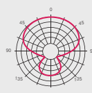
Polar Pattern
