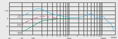
Frequency Response
